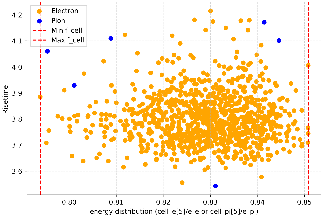
Scatter plot of f_{\text{cell}} vs risetime for energy 60.0GeV
